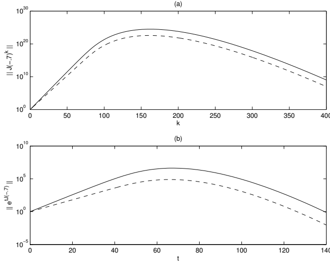
FIG. 4.1. Norms of functions of a Jordan block of size n = 50 with eigenvalue \lambda = -7 . (a) Norm of J(\lambda)^k (solid) and lower bound (4.1) (dashed), (b) Norm of e^{tJ(\lambda)} (solid) and lower bound (4.2) (dashed).
