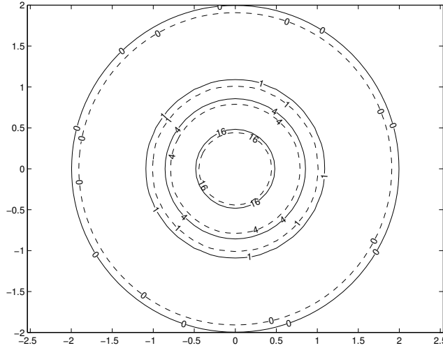
FIG. 4.2. Contour plot of the logarithm base 10 of the resolvent norm (solid) and the lower bound (4.4) (dashed) for a 50 by 50 Jordan block with eigenvalue 0.
