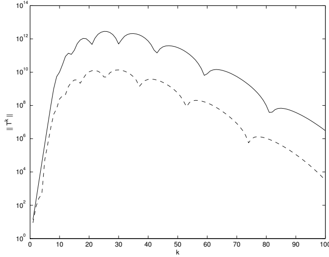
FIG. 4.3. Norms of powers of an 18 by 18 triangular Toeplitz matrix with symbol (4.5). Solid line is \|A^k\| ; dashed line is lower bound from (2.3) applied to J(0) with f(z) = [s(z)]^k .
